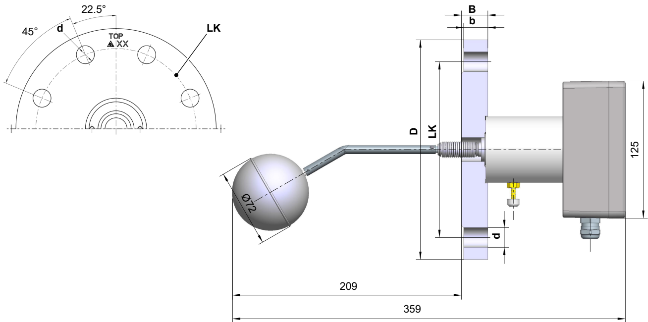
Fig. 4: Dimensional picture NK102 NK10G
